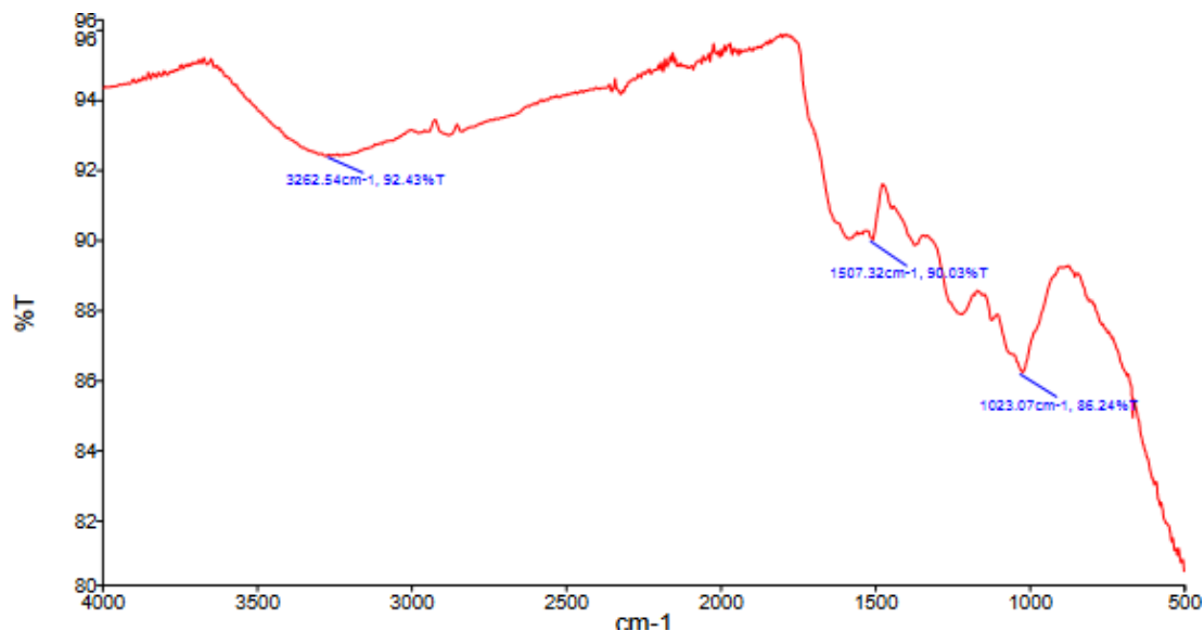
Figure 2. FTIR spectrum of Artemisia maritima -synthesized silver nanoparticles showing key absorption peaks at 3262.54 \text{cm}^{-1} ( -\text{OH} stretch), 1507.32 \text{cm}^{-1} (aromatic \text{C}=\text{C} ), and 1023.07 \text{cm}^{-1} ( \text{C}-\text{N} stretch of amines), confirming the involvement of phytochemicals in nanoparticle stabilization.
