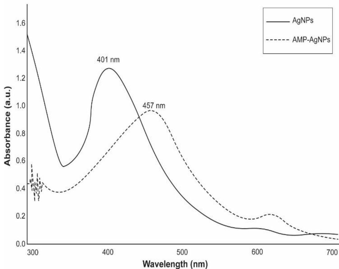
Figure 1. UV–Vis absorption spectra of biosynthesized AgNPs and ampicillin-functionalized silver nanoparticles (AMP–AgNPs). The peak at 401 nm confirms AgNP formation, while the redshift to 457 nm indicates successful ampicillin functionalization.
